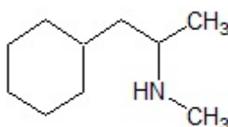
Propylhexedrine
