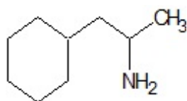
Norpropylhexedrine
